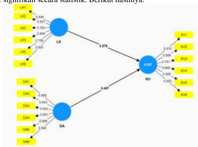
Gambar 3. Diagram Koefisien Jalur (Diagram Path Coefficients)
