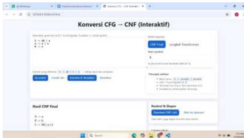
Gambar 3. Output Website
